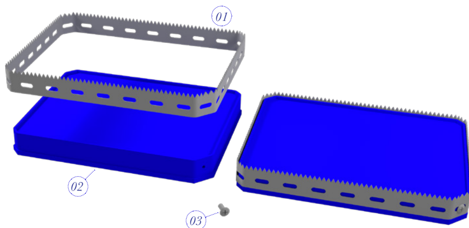
1 / Saw blade 2 / Sealing plate 3 / Fixing screw
