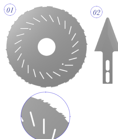
1 / Carcass cutting blade 2 / Meat cutting blade
